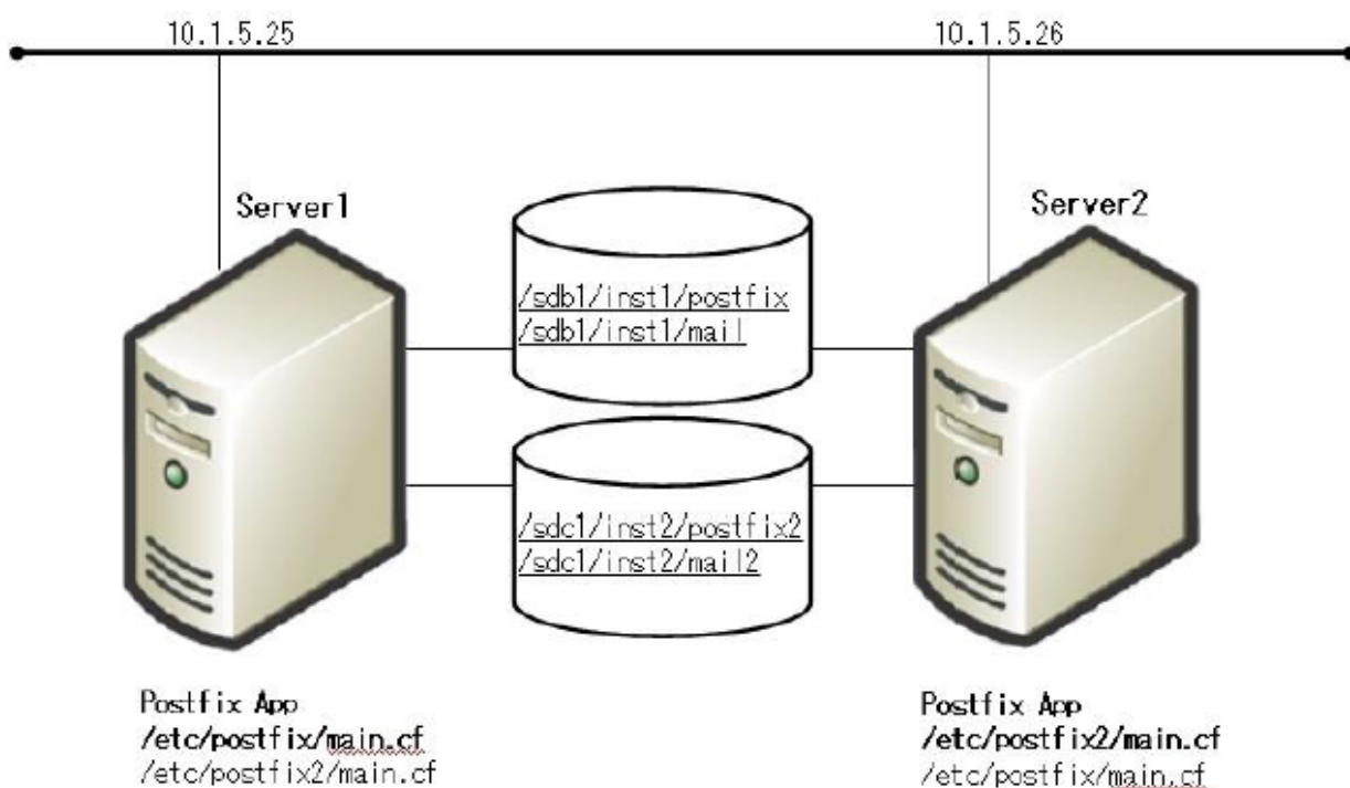
Figure 3: Typical LifeKeeper Active/Active Postfix Environment
