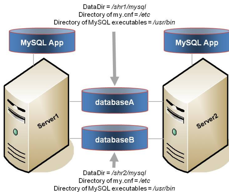
Figure 2. Active/Active Configuration, Example 2
